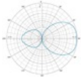
TYPICAL RADIATION PATTERN (E-PLANE)
