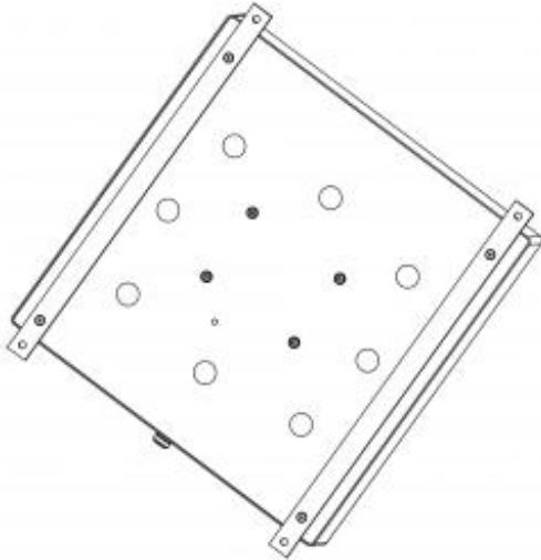
WALL MOUNTING BRACKET: PATCH-WAMO (ORDERED SEPARATELY)
