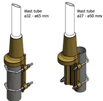
MULTI-PURPOSE MOUNTING BRACKET
